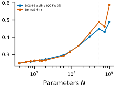
hellaswag
