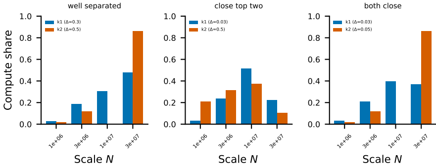
Computed challenger-allocation compute share by scale, across gap regimes
