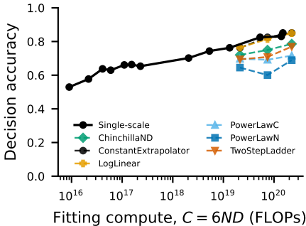
Accuracy vs. compute
