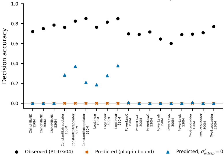
Predicted vs. observed accuracy
