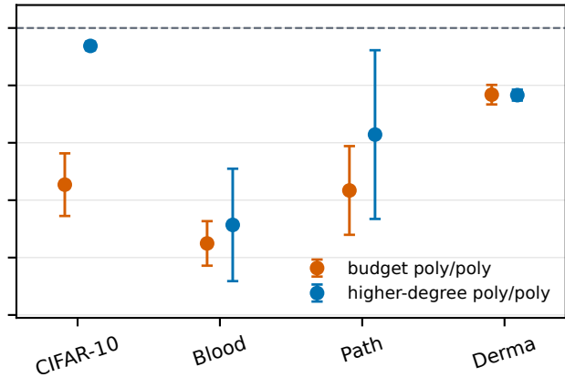
Attention-only conversion
