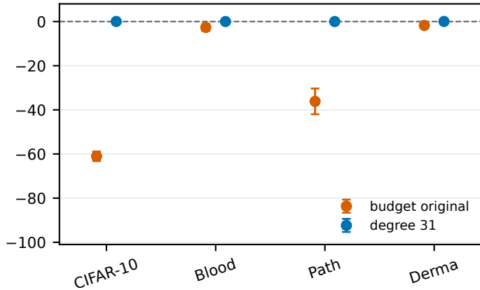
GELU-only conversion
