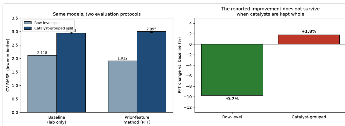
Figure 1 — The central finding. Identical models under two evaluation protocols. When every measurement of a catalyst is confined to one fold, the reported improvement inverts.
