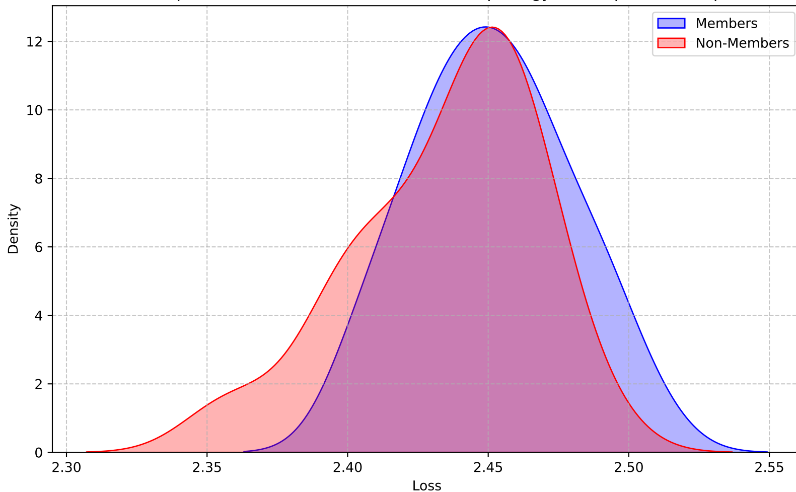
Loss Distribution Comparison (KDE), dataset=DukeData,Morphology=True,operations=open,DPSGD=True
