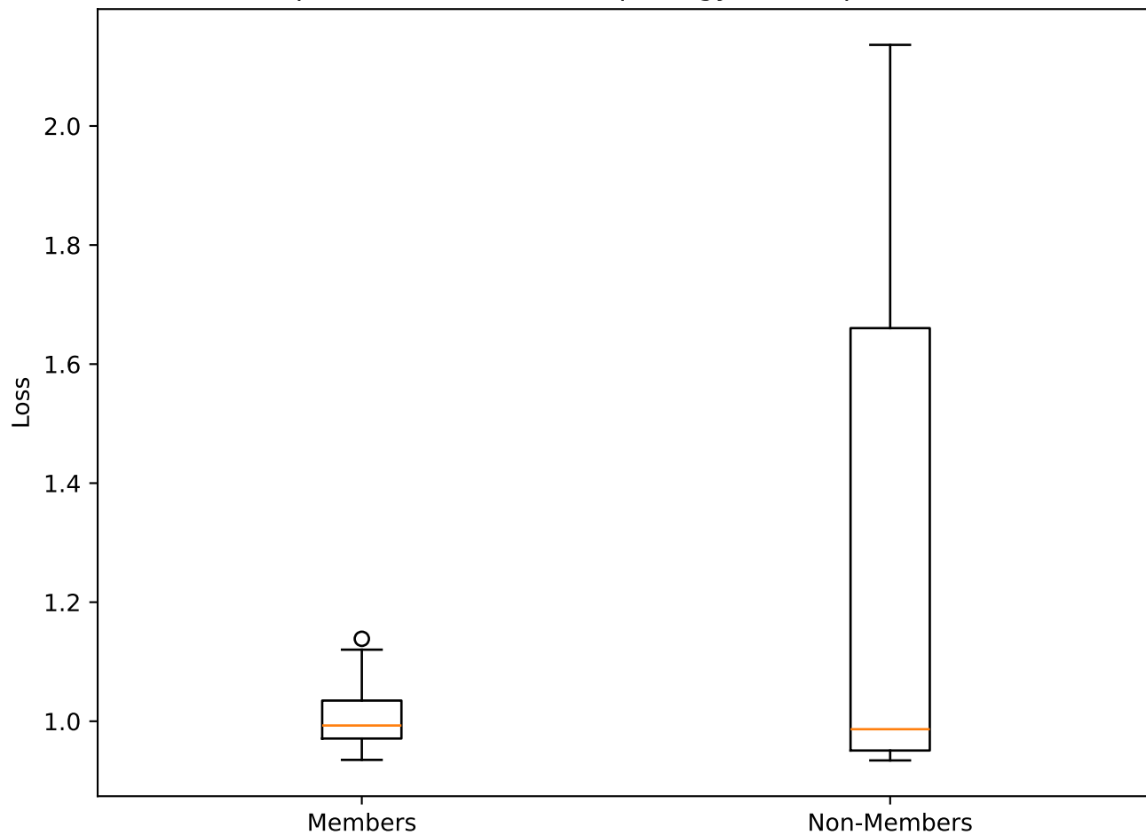
Loss Distribution Comparison (Box Plot), Morphology=True,operations=close,DPSGD=True
