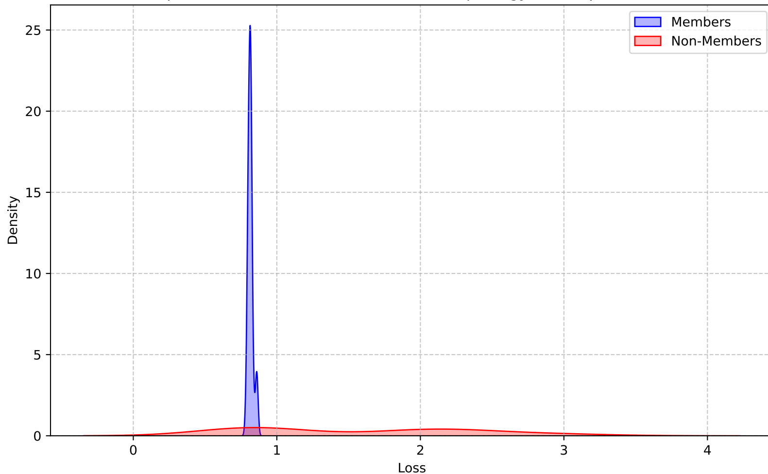
Loss Distribution Comparison (KDE), dataset=DukeData,Morphology=True,operations=close,DPSGD=False
