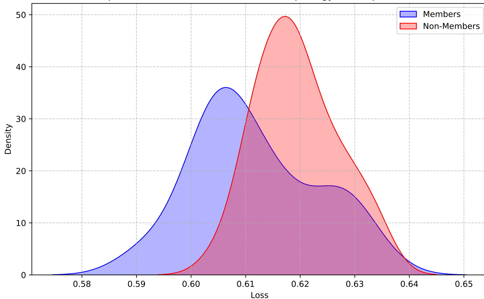
Loss Distribution Comparison (KDE), dataset=UMNData,Morphology=True,operations=close,DPSGD=True
