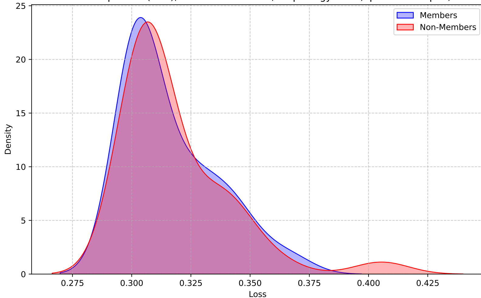
Loss Distribution Comparison (KDE), dataset=UMNData,Morphology=True,operations=open,DPSGD=True
