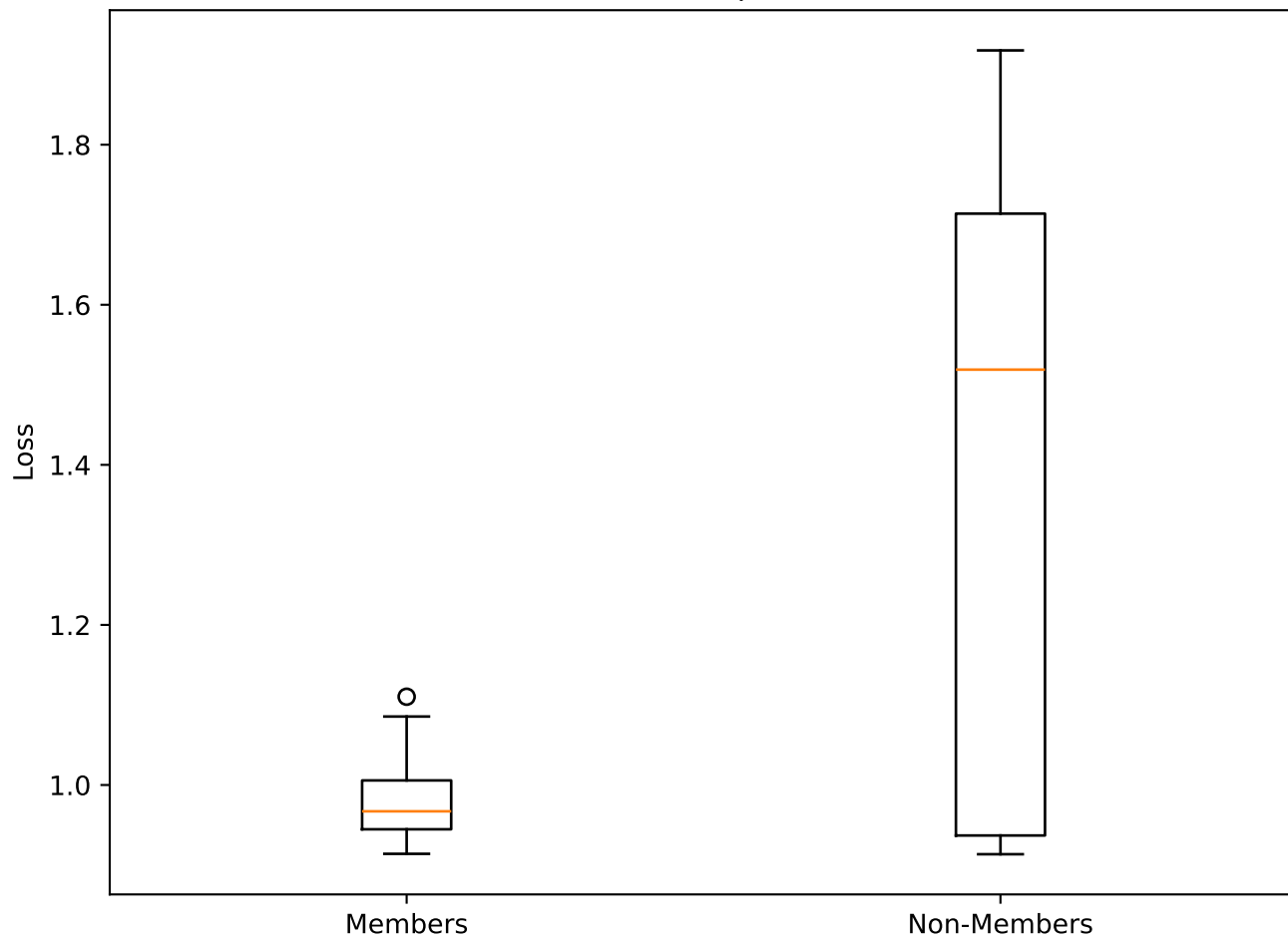
Loss Distribution Comparison (Box Plot)
