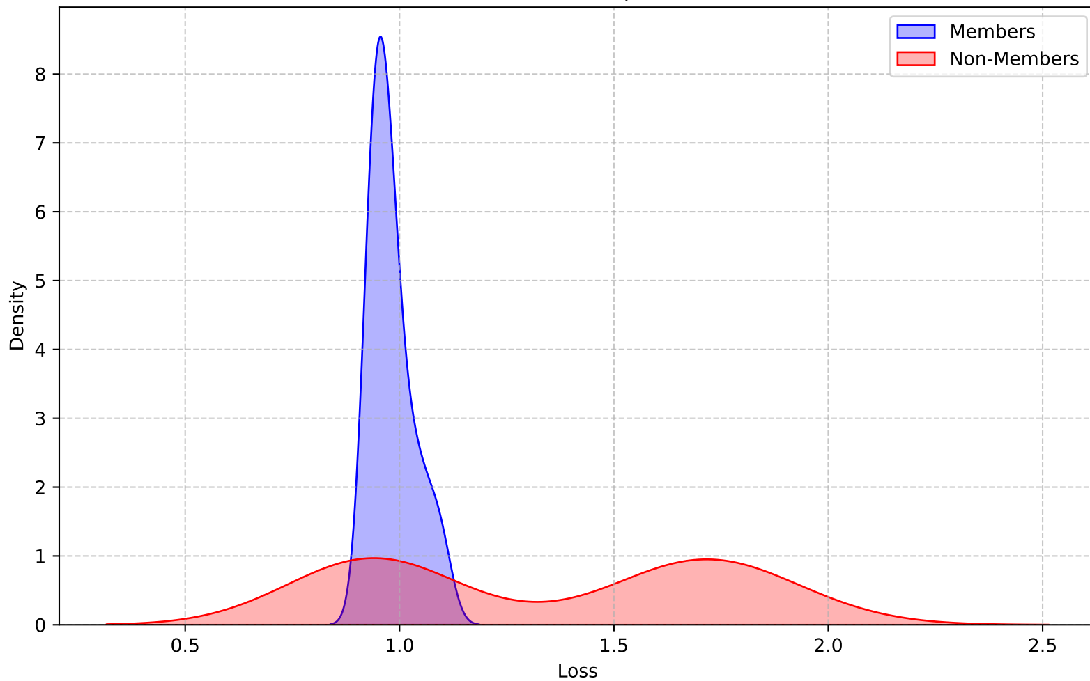
Loss Distribution Comparison (KDE)
