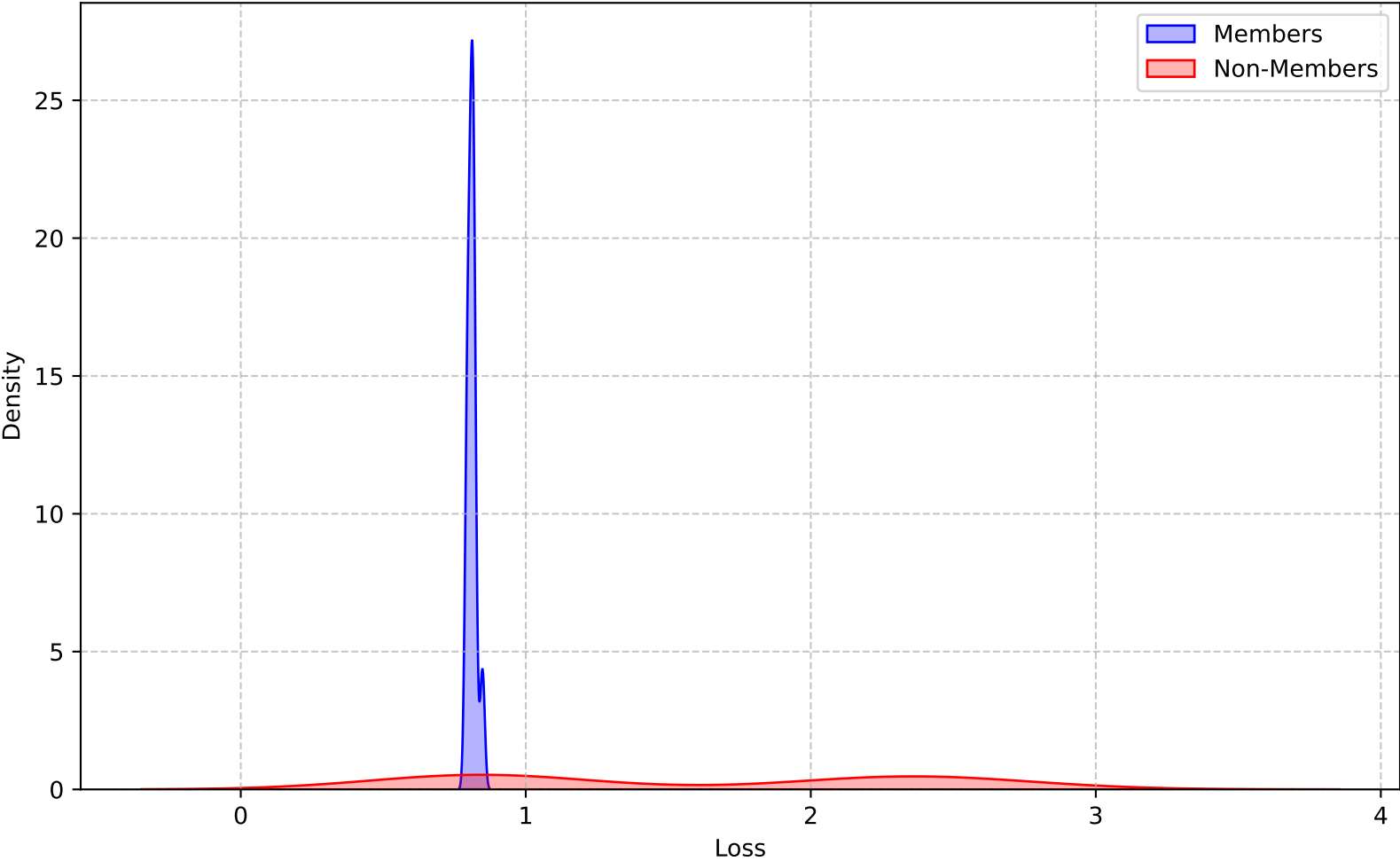
Loss Distribution Comparison (KDE), dataset=DukeData,Morphology=False,operations=close,DPSGD=False
