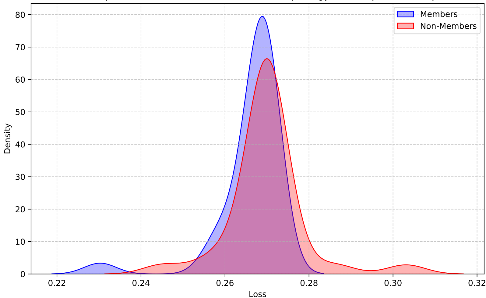
Loss Distribution Comparison (KDE), dataset=UMNData,Morphology=False,operations=open,DPSGD=True
