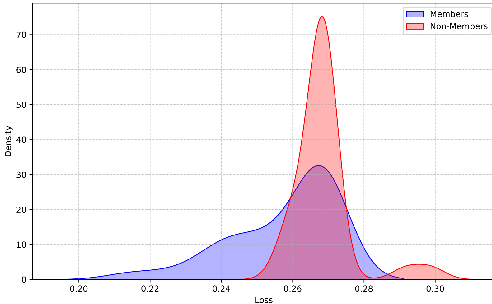
Loss Distribution Comparison (KDE), dataset=UMNData,Morphology=True,operations=both,DPSGD=False
