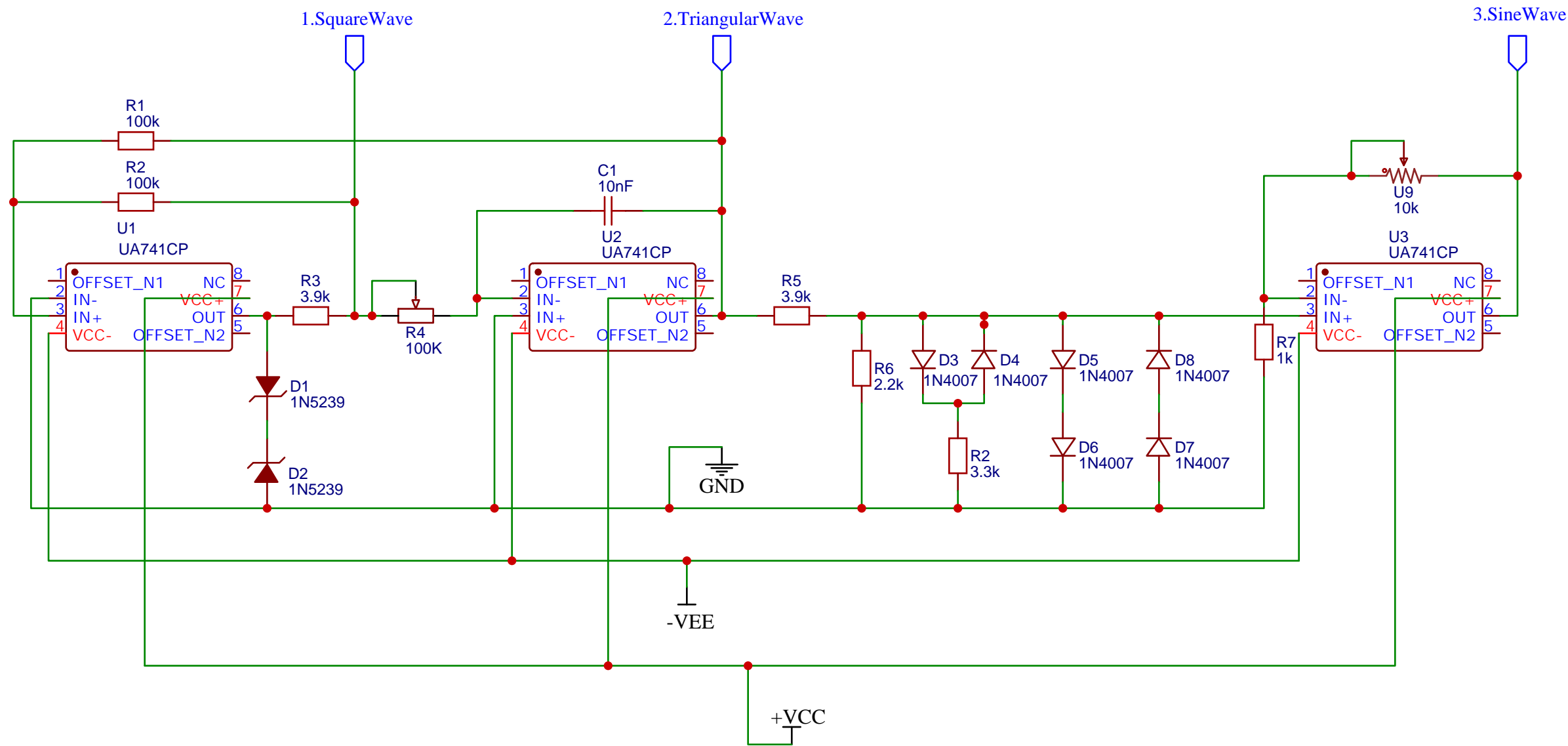
Signal Generator Using 741 Op-Amp
