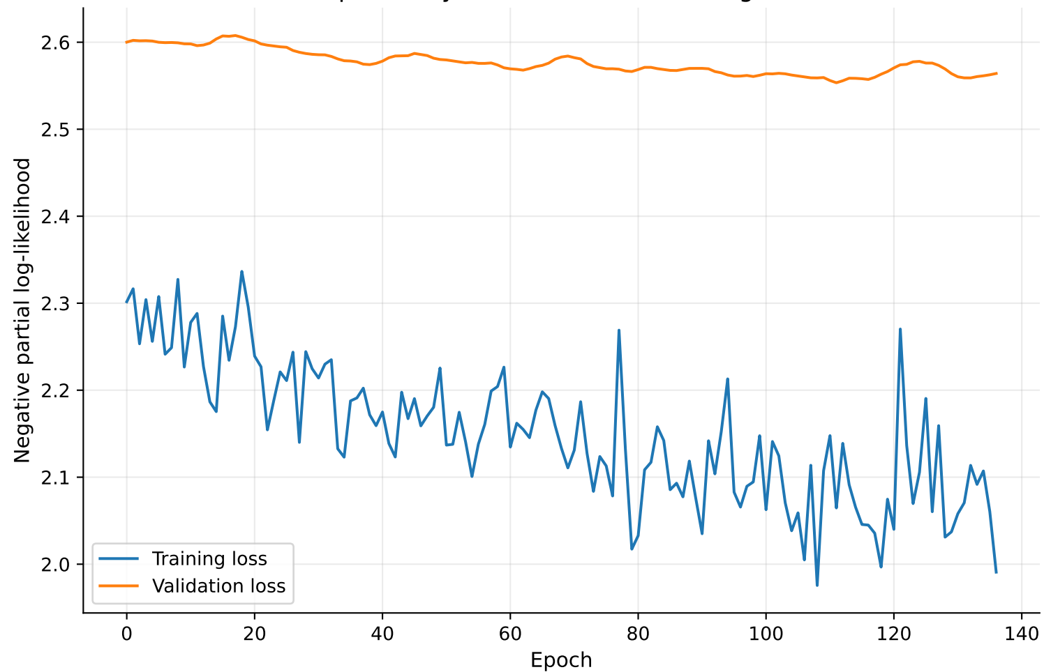
DeepSurv-Style Neural CoxPH Training Curve
