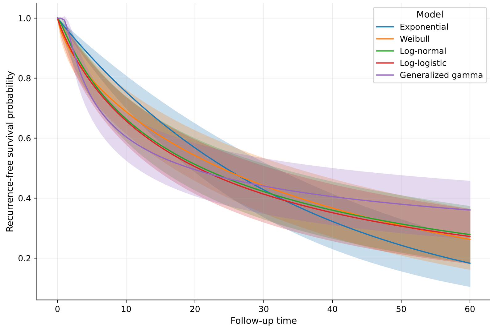
Parametric Survival Model Fits for Time to First Recurrence
