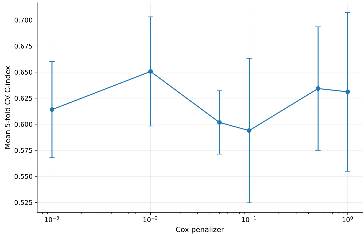
Penalized Cox Model Selection
