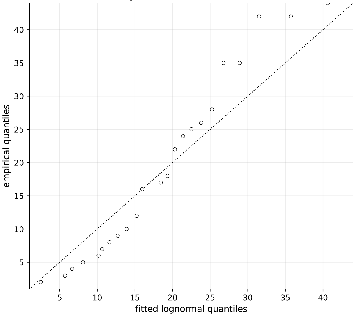
QQ Plot: Log-normal Parametric Survival Model
