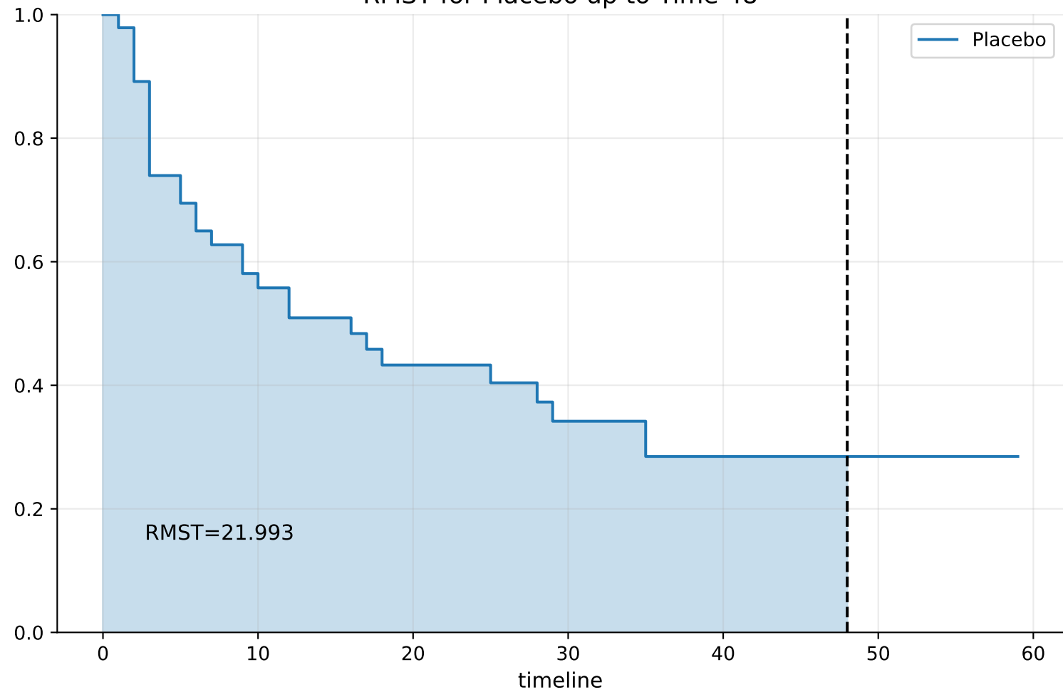
RMST for Placebo up to Time 48
