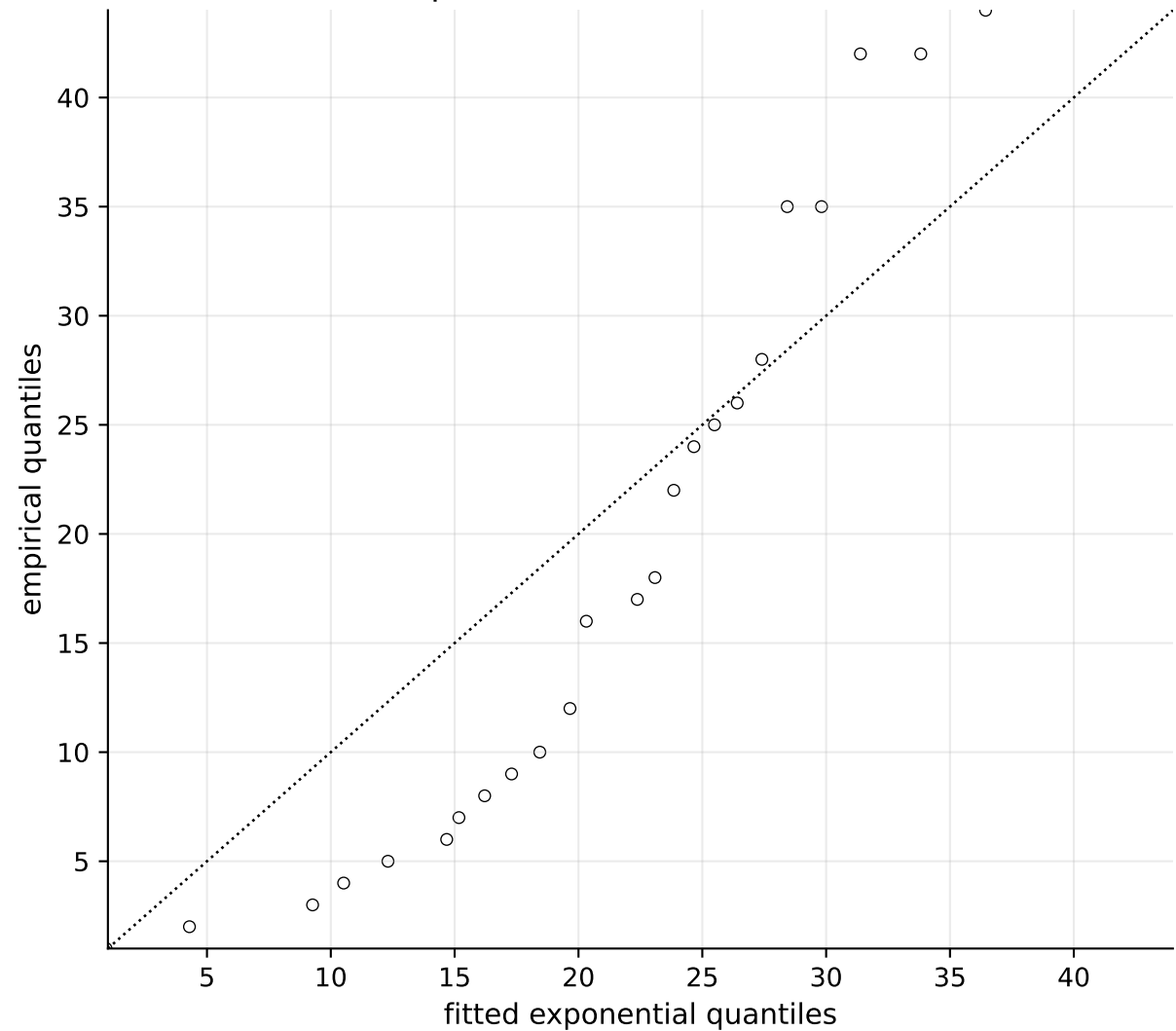
QQ Plot: Exponential Parametric Survival Model
