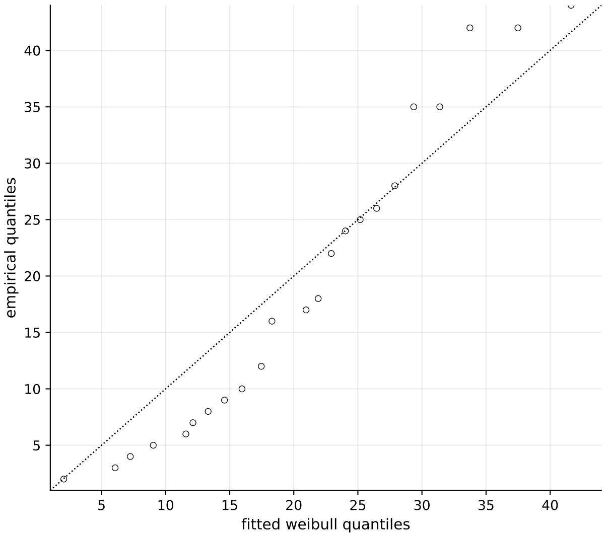
QQ Plot: Weibull Parametric Survival Model
