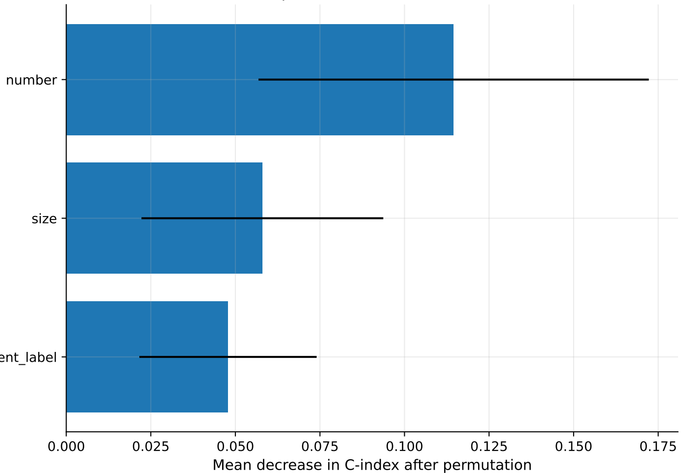
Permutation Importance for Random Survival Forest
