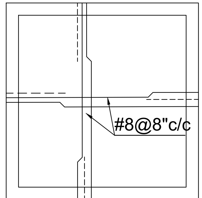
TYPICAL SLAB DETAILS
