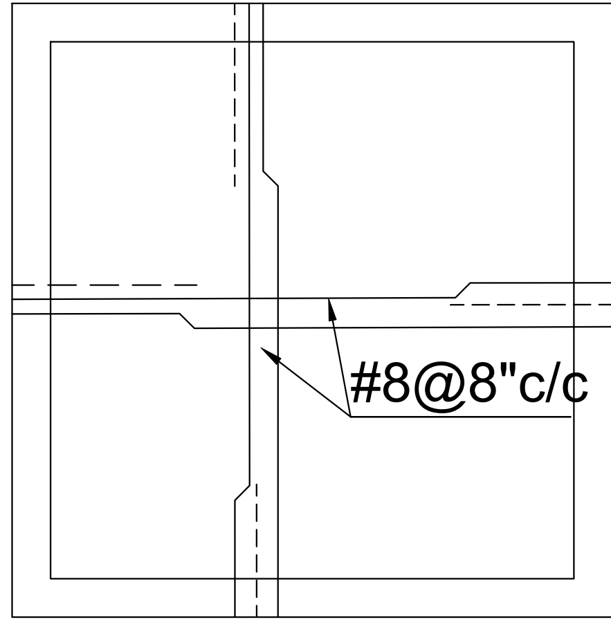
TYPICAL SLAB DETAILS
