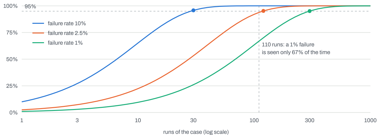
Figure 7.2 The chance of seeing at least one failure in n runs, 1 - (1 - p)^n , for three failure rates. Each dot is at 3/p runs, where the chance first reaches about 95%.
