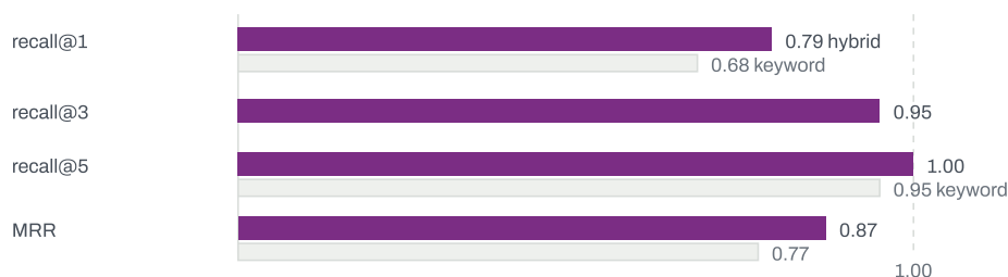
RECALL@K AND MRR, 19 LABELED QUESTIONS
