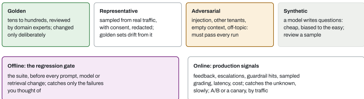
Figure 7.5 Where cases come from, and the two halves of evaluation. Keep part of the data held out and never tune against it, or the prompt overfits the eval; refresh golden sets from production, because real questions drift.
