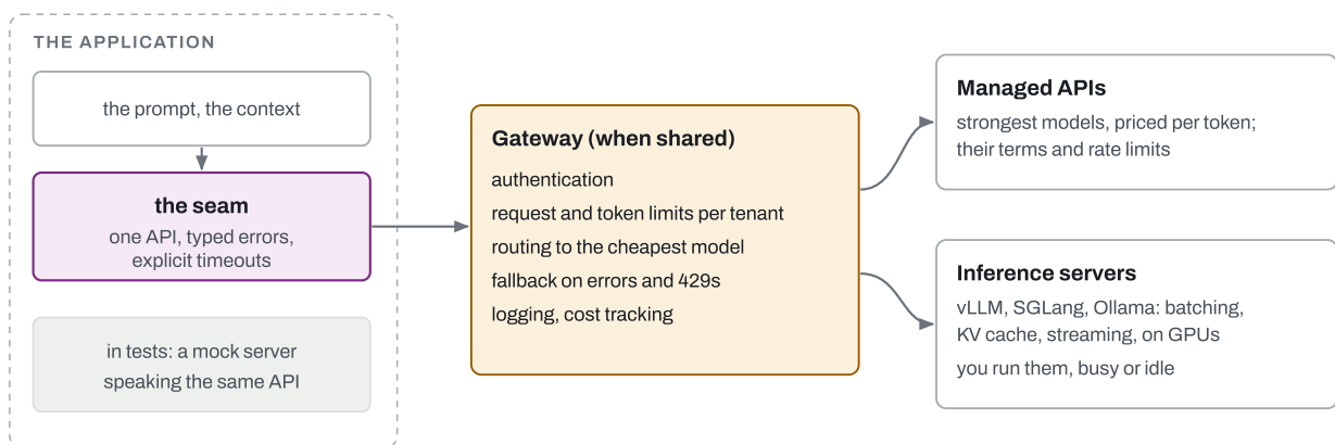
Figure 3.4 The serving path. Because the reference service's seam already speaks the OpenAI API, adding a gateway later changes one setting, the base URL. Every route a gateway can choose needs its own eval results.
