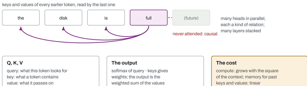
Figure 2.2 Causal attention for one token. Because a token attends only to earlier tokens, the keys and values computed for the past never change, and can be kept rather than recomputed: the KV cache.
