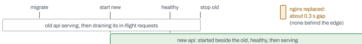
Figure 6.2 Why "recreate" is downtime. The rolling deploy failed no request during the api swap, with every in-flight stream finished. The one remaining gap is replacing the single proxy that owns the port: about 0.3 s when nginx owns it, as on the AWS VM. Behind the reference TLS edge, nginx swaps with no failed request, and the gap moves to replacing the edge itself, about 2 s, which the script does only when the edge changed. Only a load balancer in front of two hosts removes it.
