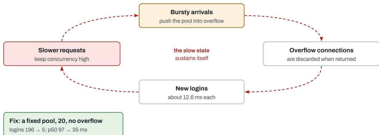
Figure 7.3 A metastable failure: a slow state kept alive by its own slowness, after the trigger is gone. Fix the feedback loop (a fixed-size pool), not only the trigger.
