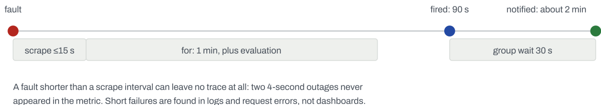
Figure 14.4 How long the reference stack takes to notice a failure, measured end to end with the rate limiter's store stopped. Every alert rule also has unit tests that feed it synthetic series and assert when it must and must not fire.
