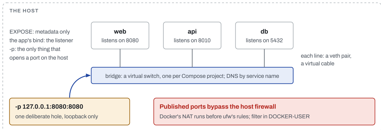
Figure 12.3 How a Compose stack is wired on one host. Service names resolve only within one host's Docker networks; spanning hosts is the job of an orchestrator, which is the real reason Kubernetes and ECS exist (Handbook 3, Chapters 9 and 10).
