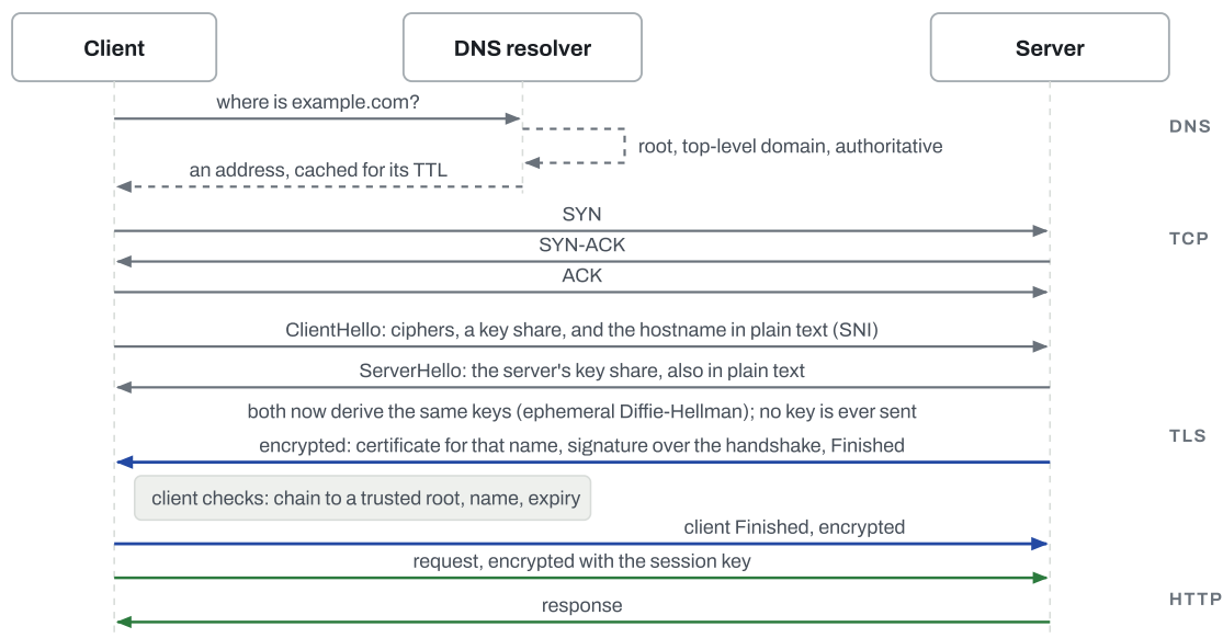
Figure 4.2 The first request to a site, in order, with TLS 1.3. A raw IP address skips DNS; a kept-alive connection skips TCP and TLS for later requests. The key shares ride in the first two messages, so the handshake takes one round trip and the certificate already travels encrypted. SNI is why one address can serve many certificates, and it is sent before anything is encrypted.
