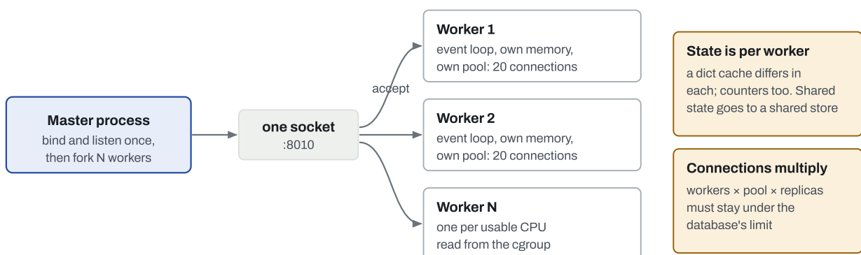
Figure 5.3 The pre-fork model. ss -ltnp shows one listening socket with N process IDs. The kernel distributes connections; the costs are per-worker memory and per-worker connection pools.
