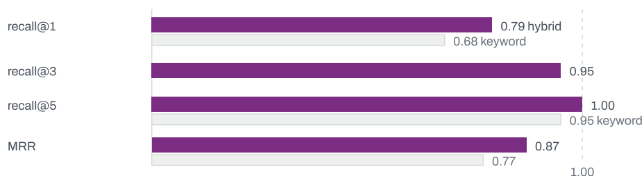
RECALL@K AND MRR, 19 LABELLED QUESTIONS
