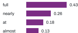
TEMPERATURE 1.5: FLAT
