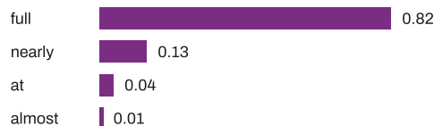
TEMPERATURE 0.3: SHARP
