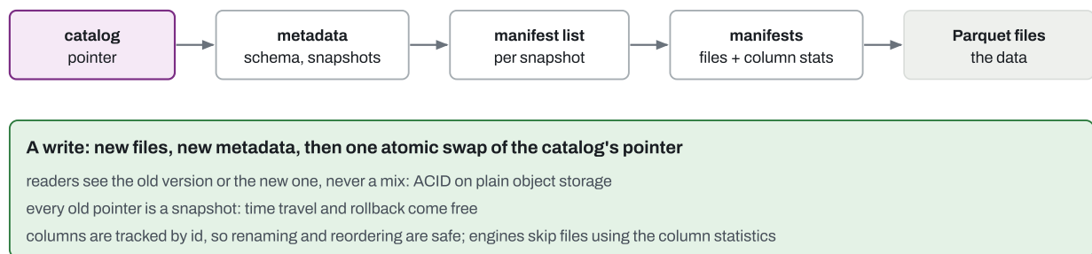
Figure 13.2 Why a table format exists: a folder of Parquet files has no atomic commit, so readers could see half-written data, and schema changes and deletes were painful. The catalog's essential job, for Iceberg, is that atomic pointer swap.
