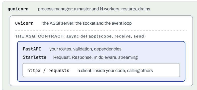
Figure 5.1 The stack of a Python web service. The reference api runs FastAPI under uvicorn workers managed by gunicorn in production, and plain uvicorn with auto-reload in development.
