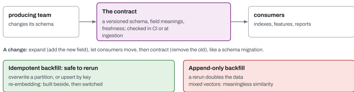
Figure 14.2 Contracts and backfills. A table format tracking columns by id makes a rename safe in storage; consumers still break, which is what the contract is for.
