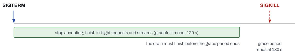
Figure 3.2 The order of a graceful stop. The application's own drain time must be shorter than the platform's grace period (Compose stop_grace_period , ECS stopTimeout , Kubernetes terminationGracePeriodSeconds ), or the kill arrives mid-answer.
