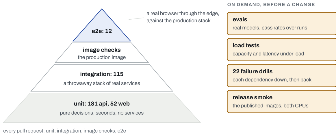
Figure 13.1 The reference service's test layers, with their sizes. Everything on the pyramid runs in CI on every pull request; the layers on the right need real models, a production-sized stack or a published release, and run before the kind of change they protect.
