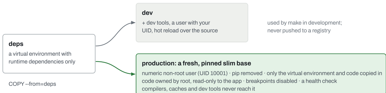
Figure 12.2 Three stages, one Dockerfile. The dev and production images share the exact dependency set, because both come from the same deps stage and lockfile.
