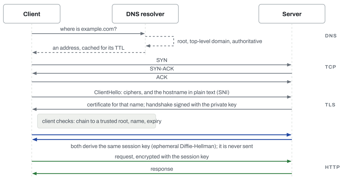
Figure 4.2 The first request to a site, in order. A raw IP address skips DNS; a kept-alive connection skips TCP and TLS for later requests. SNI is why one address can serve many certificates, and it is sent before anything is encrypted.
