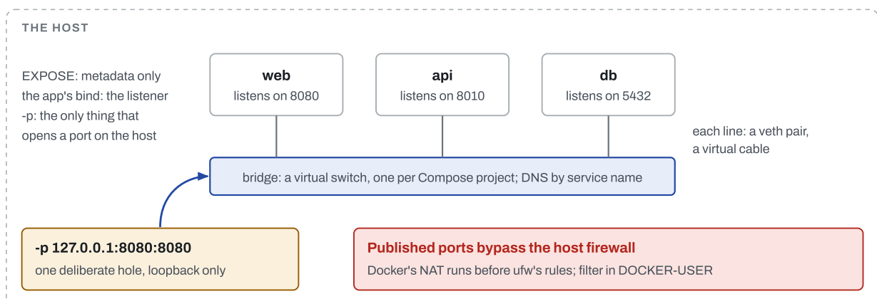
Figure 12.3 How a Compose stack is wired on one host. Service names resolve only within one host's Docker networks; spanning hosts is the job of an orchestrator, which is the real reason Kubernetes and ECS exist (Handbook 3, Chapters 9 and 10).
