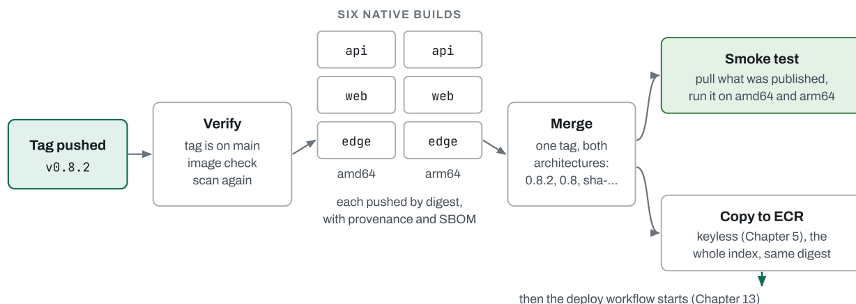
Figure 3.2 The release workflow. It builds each image once per processor type, joins them under the release tags, and then tests what it published, not what it built. Only after that are the images copied onward and deployed.
