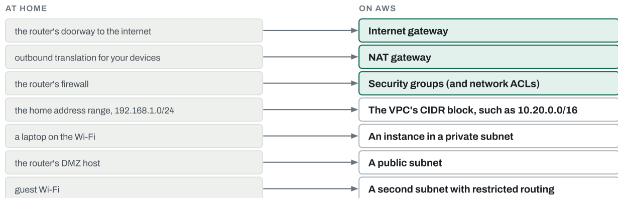
Figure 8.1 The home router's jobs, and their AWS equivalents. On AWS each job is a separate resource, which is why a cloud network has more parts to configure but also more control.
