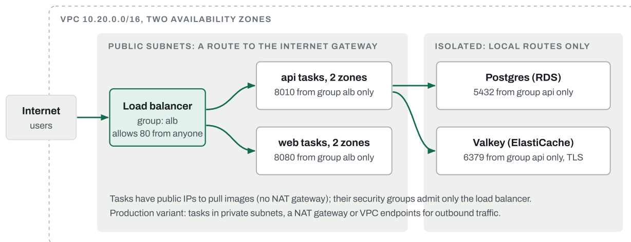
Figure 8.2 The reference network. Security groups name each other in a chain: internet to load balancer, load balancer to tasks, api to data. A task added by autoscaling joins its group and is covered without any rule changing.
