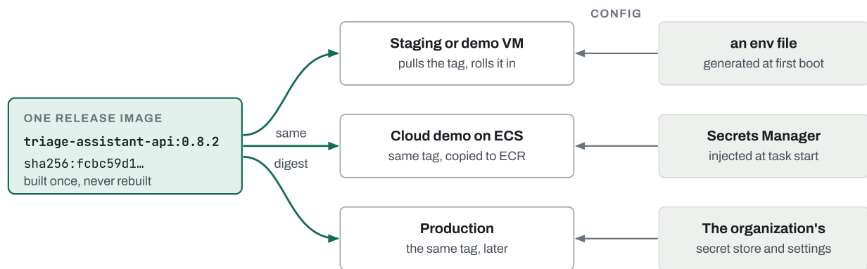
Figure 1.2 The image is the constant; the configuration is the variable. Because nothing environment-specific is baked into the image, a problem found in staging is a problem in the exact bytes production would run.
