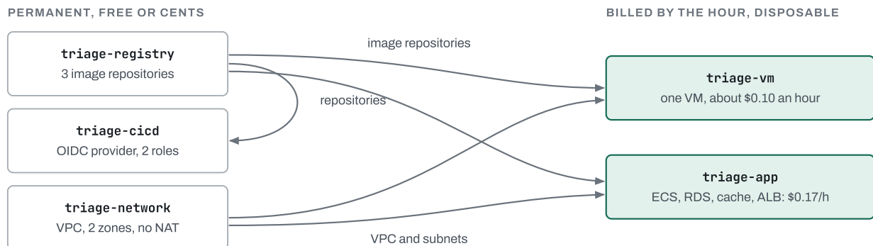
Figure 7.2 Stacks split by lifetime. Each arrow is a cross-stack reference, which CloudFormation implements as an export from the producer and an import in the consumer: the producer must be deployed first, and cannot delete what a consumer still imports.
