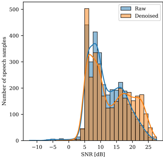
SNR Distribution - Raw and Facebook Denoiser
