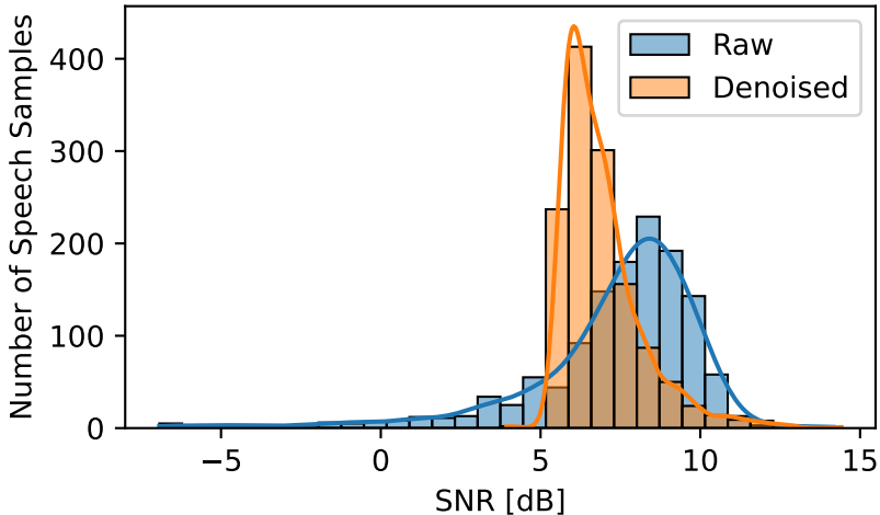
SNR Distribution - M
