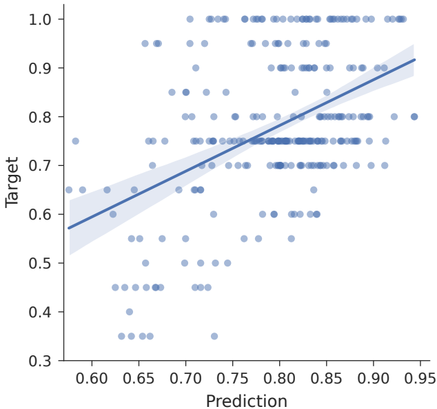
Regression Plot
