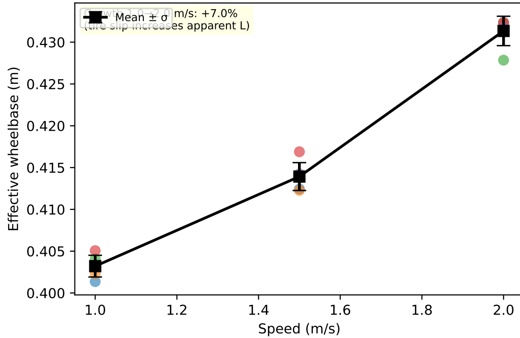
Wheelbase vs. Speed (tire slip effect)
