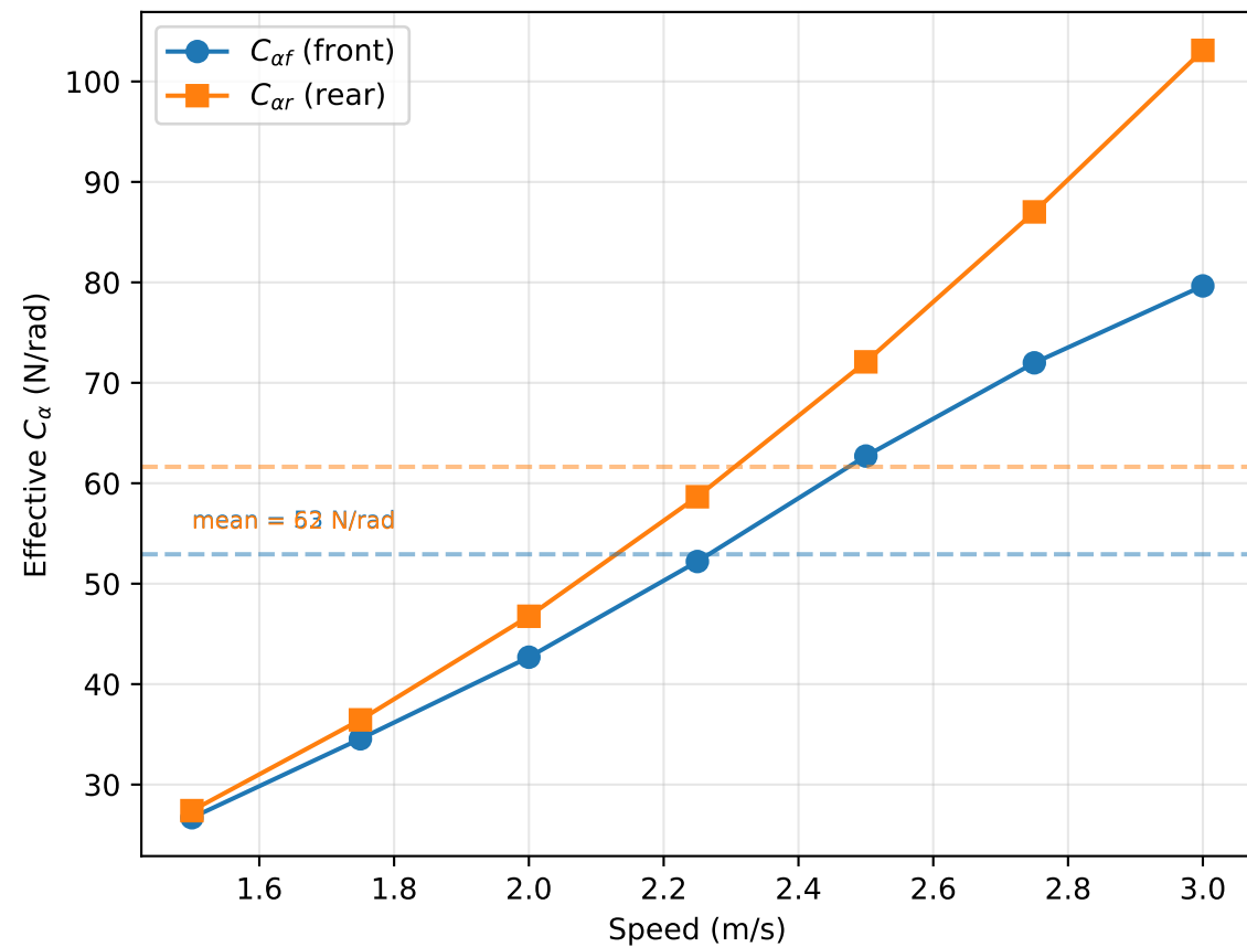
Effective C_\alpha vs. Speed
