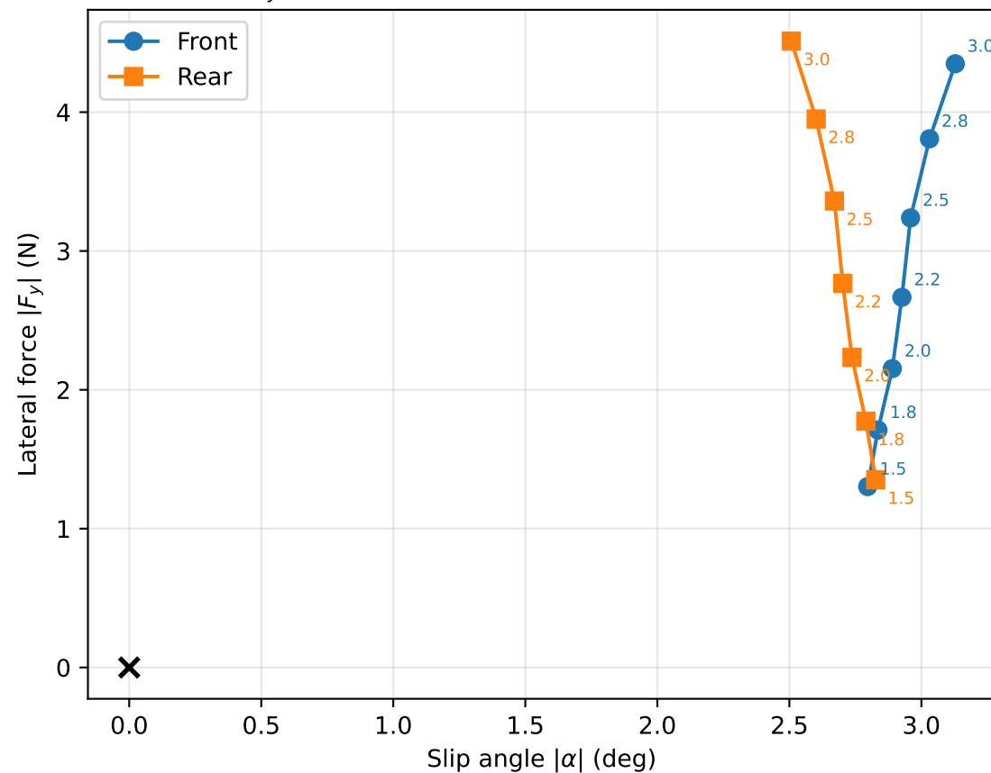
F_y vs. Slip Angle (speed annotated, m/s)
