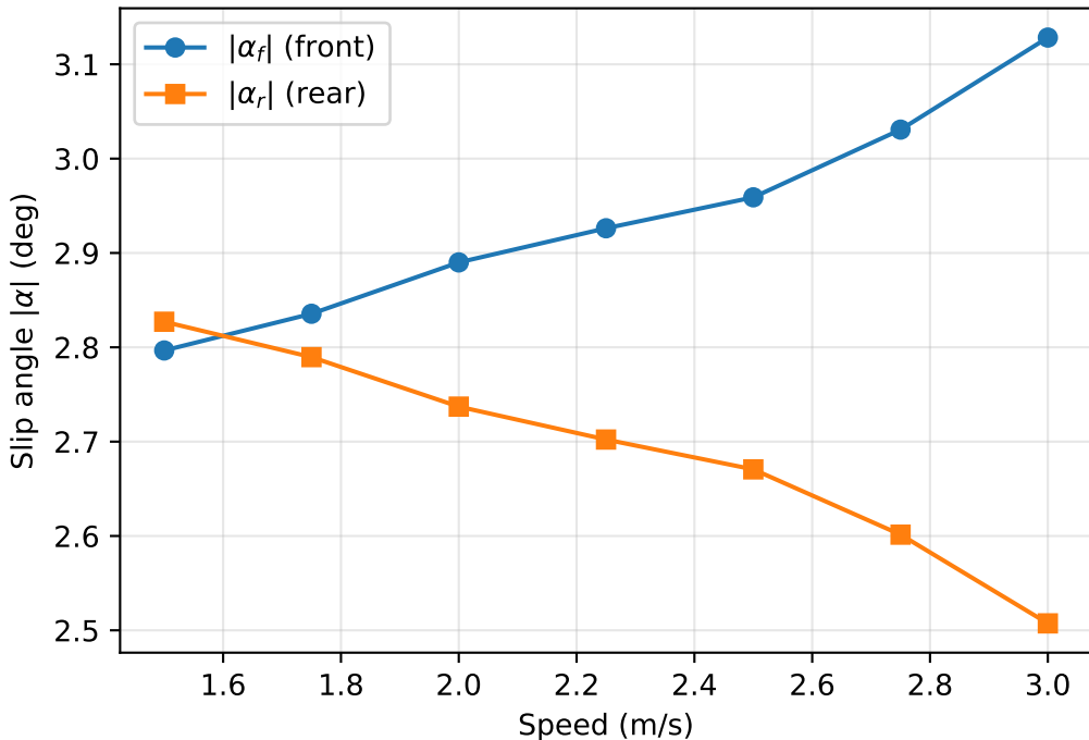
Slip Angle Growth with Speed
