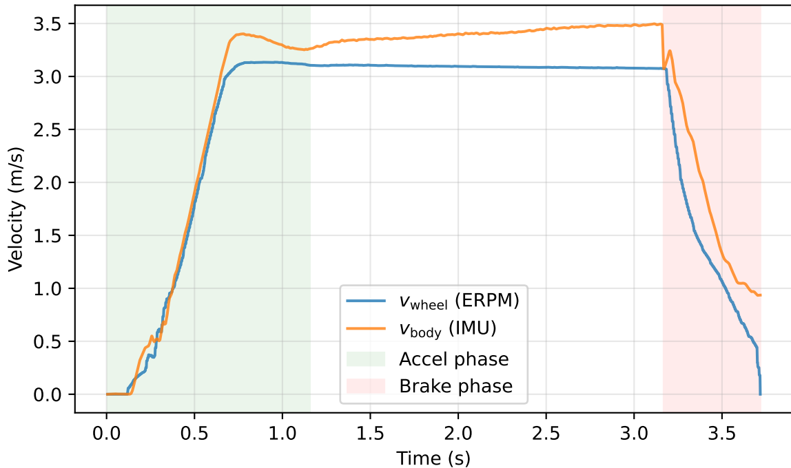
Wheel Speed vs. Body Speed — Longitudinal Slip
