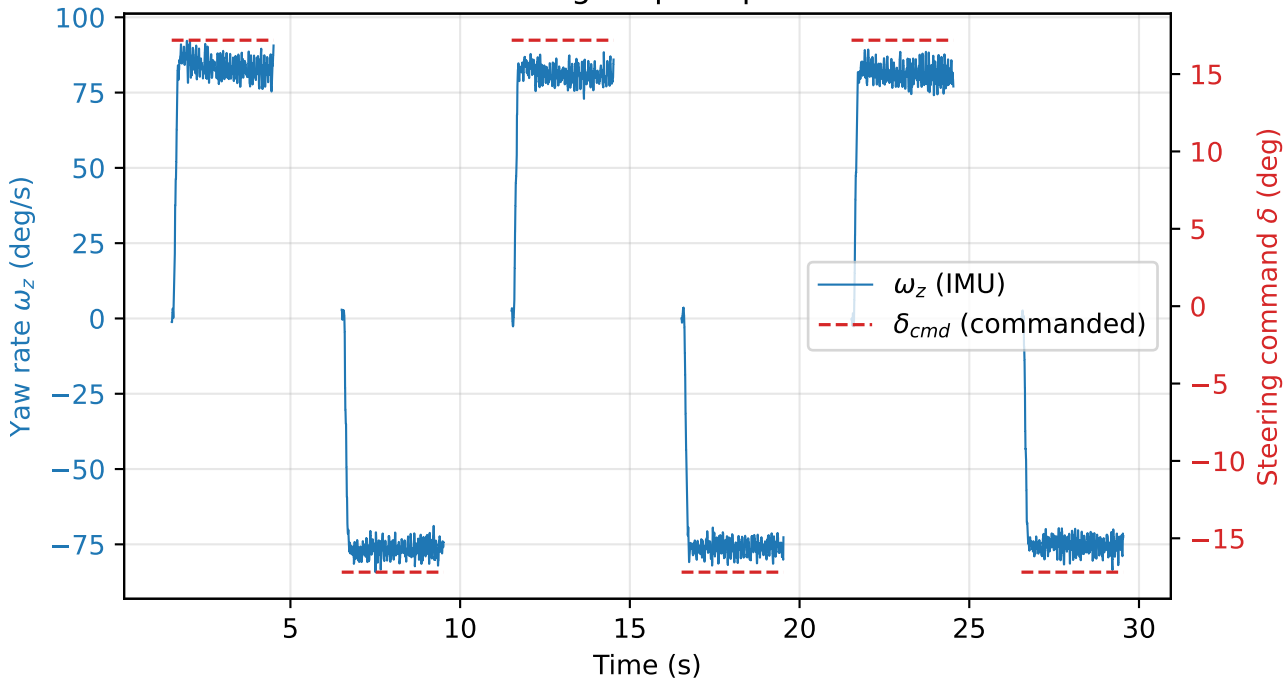
Steering Step Response
