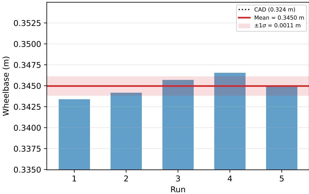
Per-Run Consistency (v = 1.0 m/s)
