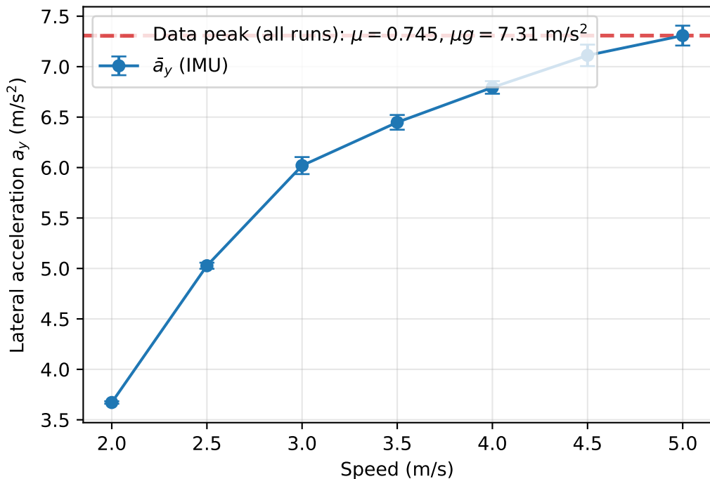
Friction Coefficient Identification (5 runs)
