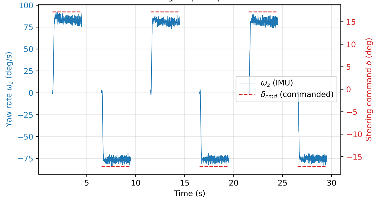
Steering Step Response
