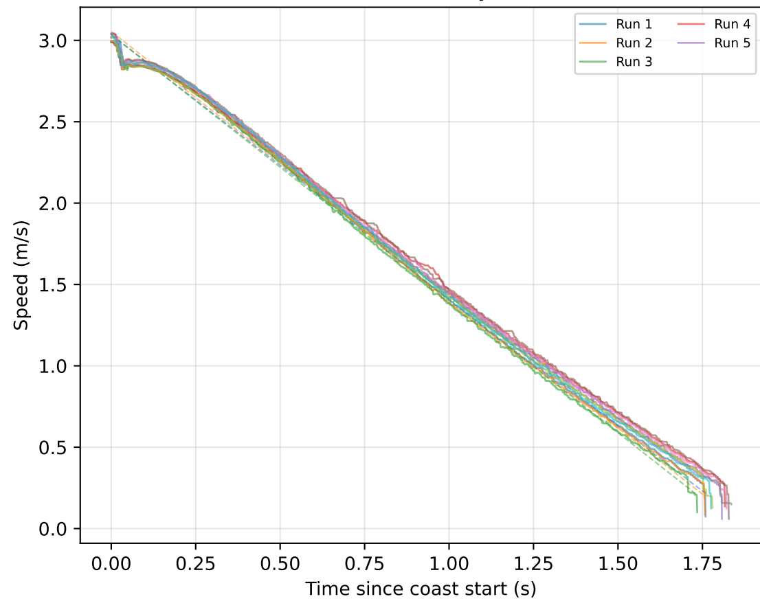
Coast-Down Velocity Profiles
