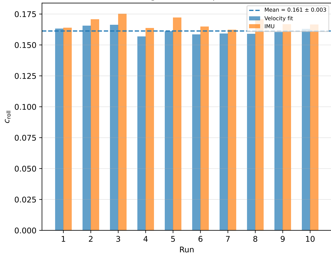
Rolling Resistance per Run
