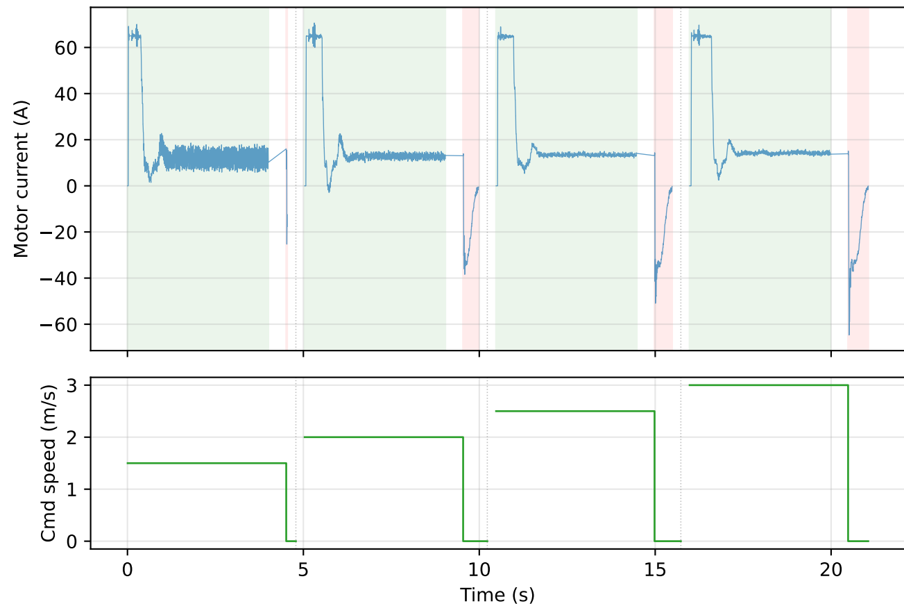
Motor Current vs. Time
