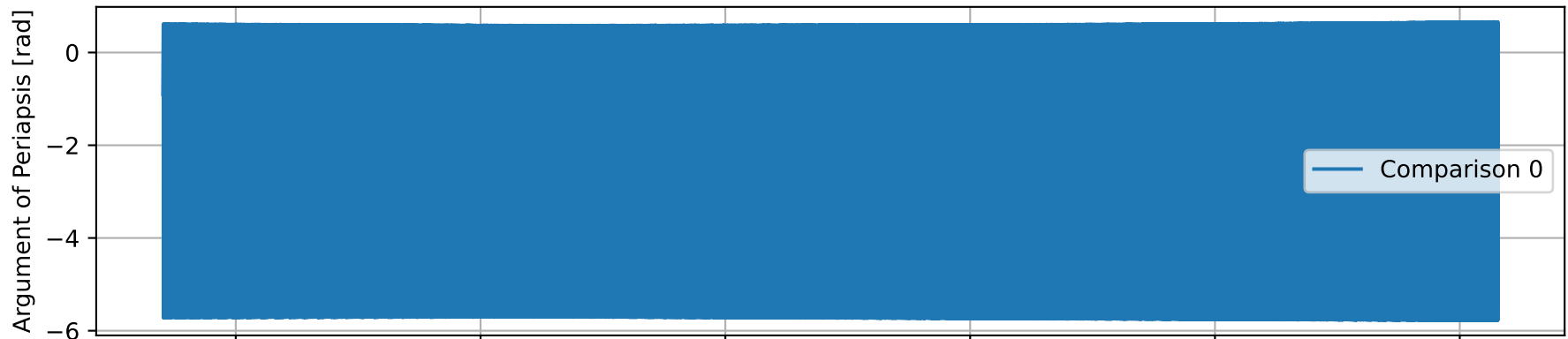
Difference in Keplerian State for Triton Spice w.r.t. Neptune (Component 4)
