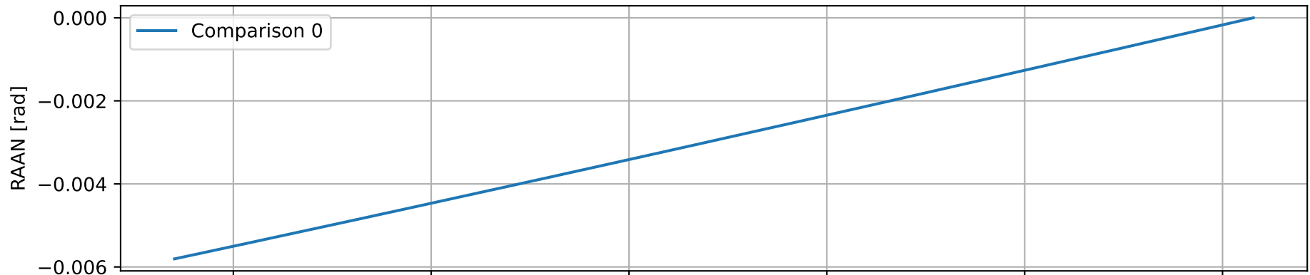
Difference in Keplerian State for Triton Spice w.r.t. Neptune (Component 5)
