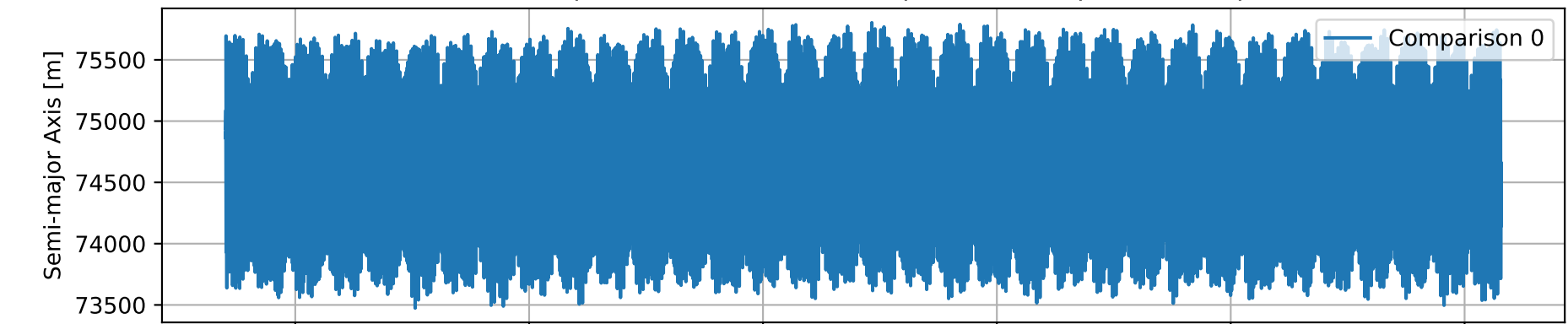
Difference in Keplerian State for Triton Spice w.r.t. Neptune (Component 1)
