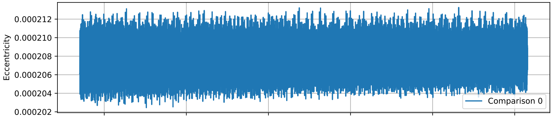
Difference in Keplerian State for Triton Spice w.r.t. Neptune (Component 2)
