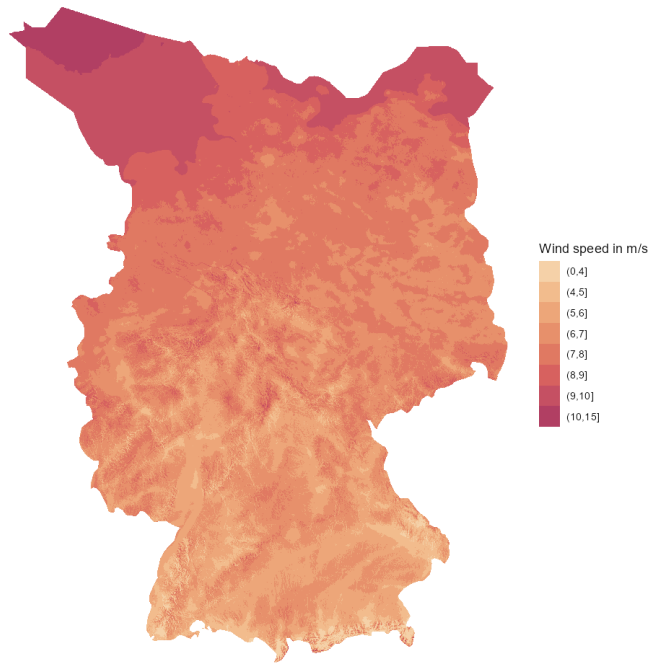
Figure 1. Average wind speed on- and offshore at a height of 100 meters
