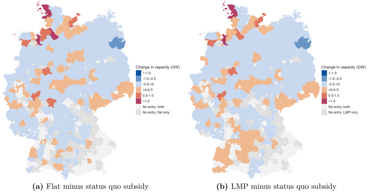
Figure 4. Change in onshore wind capacity under alternative subsidy designs
