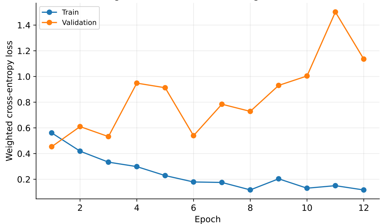
Single-frame ResNet18 learning curve: loss
