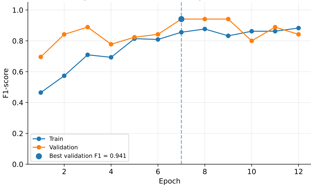
Single-frame ResNet18 learning curve: F1-score
